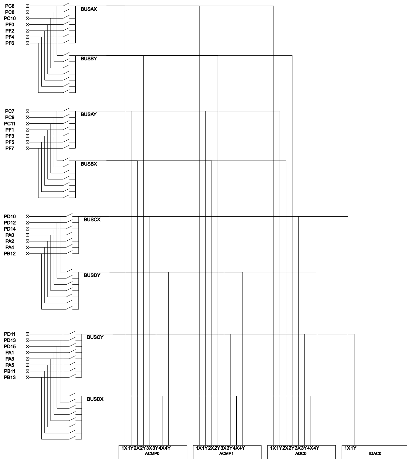
Figure 7.2. BGM11S APORT
